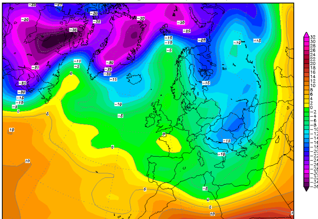
Figure 11. Thermal field at the level from the altitude of 850 hPa on January 25, 1963, at 00 UTC, at the level of 2m altitude at the moment of the maximum intensity of the second big cold wave over Romania (according to Wetterzentrale - Kartenarchiv)
