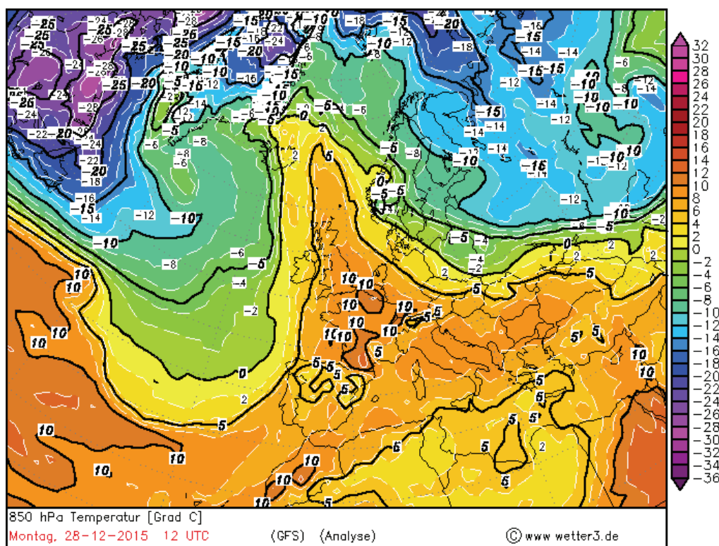
Figure 6. Thermal field in altitude at the level of 850 hPa (at the average height of 1500 m) on December 28, 2015 at 12 UTC (according to http://www1.wetter3.de/Archiv/ ).
